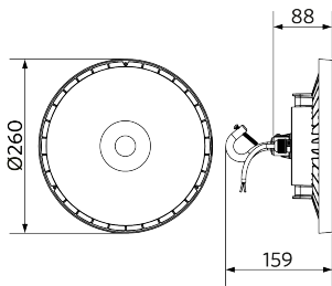
Dimensional_Drawing_HB_E3_70W.png
