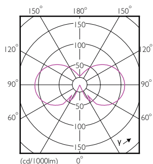
Light Distribution Diagram - CorePro LEDLuster ND 2.2-25W P45 E27 FRG
