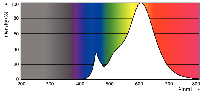
Spectral Power Distribution Colour - CorePro LEDbulb ND 8-60W A60 E27 827
