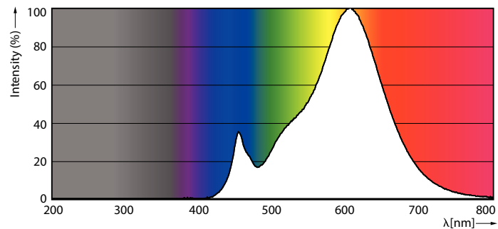
Spectral Power Distribution Colour - CorePro LEDbulb ND 8-60W A60 E27 827 SKT
