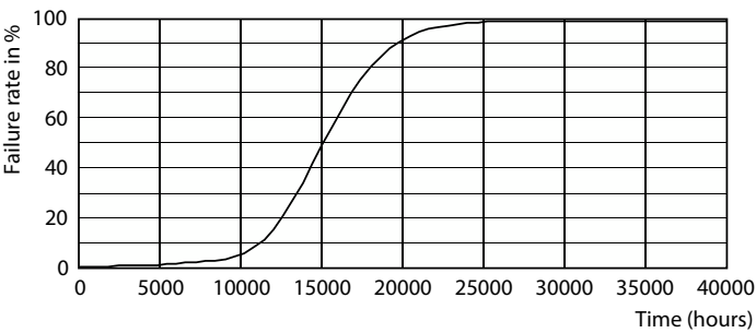
Life Expectancy Diagram - CorePro LEDBulbND 120W E27 A67 827 CL G
