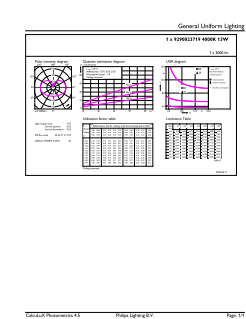
General uniform lighting - CorePro LEDBulbND 120W E27 A67 840 FR G
