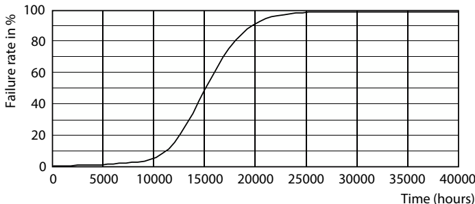
Life Expectancy Diagram - CorePro LEDCandleND6.5-60WB35 E14 840FRG
