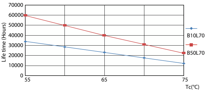
Life Expectancy Diagram - MAS LEDtube HF 600mm HO 10.5W 865 T5
