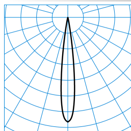
Faciella Slim 30 RE5R/2000-830 3G1 TX120344 ■ C0 - C180
