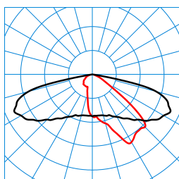
LIQ 50N-AB2L-LRA/2600-722 4G1 ETDD (CLO initial value) TX776051
