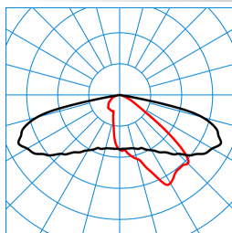
LIQ 50N-AB2L-LRA/2600-722 4G1 ETDD (CLO end value) TX776050
