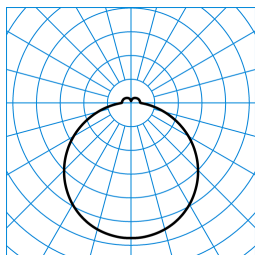
Olisq Act RWD2 DW 20 ETDD8 IP54 PC (ActDSU) TX376221
