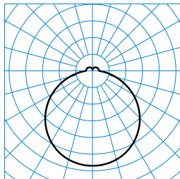
Olisq Act RWD2 DW 20 ETDD8 IP54 PC (ActDCW) TX375691
