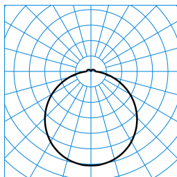
Olisq Act RWD2 DW 20 ETDD8 IP54 PC + Olisq RWD2 ZDR 1/2 03 (ActDWW) TX427705
