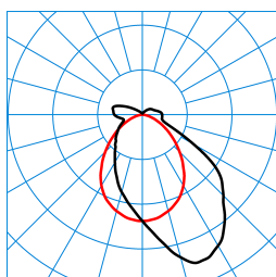
TugraHE Act 18 PAW 70-840 ETDD8 01 (ACTDCW) TX303169
