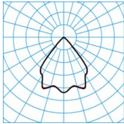
ELINE HE CLW2230-85 ML 840 L150 0 20 ■ C0 - C180
