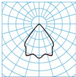
ELINE HE CLW2230-85 ML 840 L150 2 20 ■ C0 - C180
