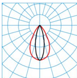
ELINE HE LEN100 840 L225 4 50
