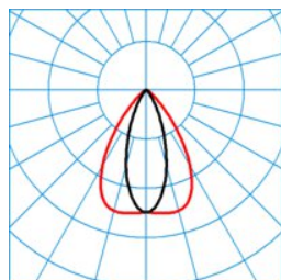
ELINE LVN55-140 ML 840 L225 2 20
