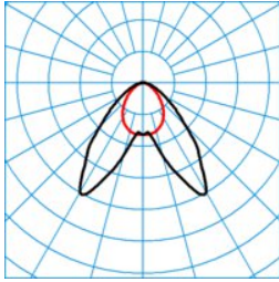
ELINE HE LDAH40-120 ML 840 L150 2 50 ■ C0 - C180 DIN 5040 = A40 UGR I 3 = 23,9 UGR q 3 = 26,0 UTE 3 = 0.98 D + 0.02 T 0.50 1.40 CEN flux code = 57 87 97 98 100 0 6 44 2
