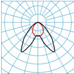
ELINE HE LDAH40-120 ML 840 L150 4 50 ■ C0 - C180 DIN 5040 = A40 UGR I 3 = 24,5 UGR q 3 = 26,6 UTE 3 = 0.98 D + 0.02 T 0.50 1.40 CEN flux code = 57 87 97 98 100 0 6 44 2
