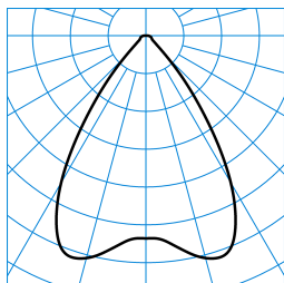
InperiaL G2 C07 BR19 1000-830 01 + ZN-PC ■ C0 - C180 TX052555
