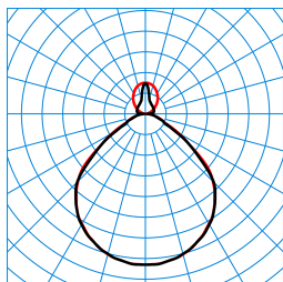
Luceos D/H2-L CDP 6500-840 03 (Ceiling D2 ZD/03) TX194614
