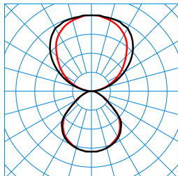
Luceos D/H2-L CDP 6500-840 03 (Pendant ZS/ZST) TX194608
