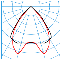
SFlow-Act D3-L MRX 40-8 ETBLE +CAS-S 01 (ACTDWW) TX711690
