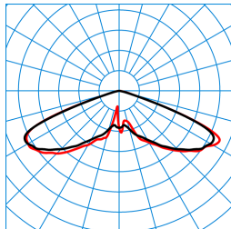
Publisca P2-RB6L/2000-730 3G1S ETDD (CLO initial value) TX301295
