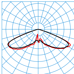
Publisca P2-RB6L/2000-730 3G1S ETDD (CLO end value) TX301916
