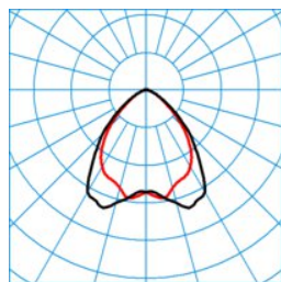
ELINE HE LW40-120 ML 865 L150 2 50 ■ C0 - C180
