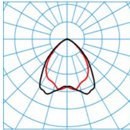
ELINE HE LW40-120 ML 865 L150 2 50
