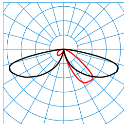
LTX PT-AB2L-LRA/15/18/26-740 4G1 (2600 lm) TX084152
