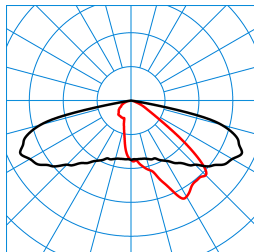
LIQ 50N-AB2L-LR-SLR2/4200-730 4G1 ET (CLO initial value) TX777122
