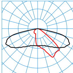
LIQ 50N-AB2L-LR-SLR2/4200-730 4G1 ET (CLO end value) TX777117
