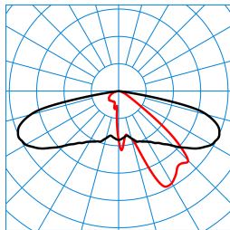
Publisca P2-AB2L/2000-740 3G1S ETDD (CLO end value) TX300242
