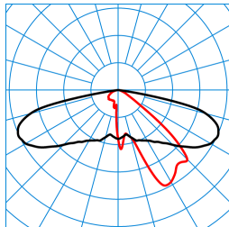
Publisca P2-AB2L/2000-740 3G1S ETDD (CLO initial value) TX301083
