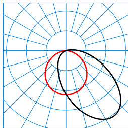
Sanesca W3-S1/R LED5000-830 01 (reading light) TX055776
