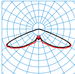
Publisca P1W-RB6L-LR/3200-740 4G1S TX053534
