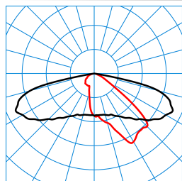
LIQ 50N-AB2L-LRA/22/26/32-722 4G1 ETDD (CLO end value) TX778453
