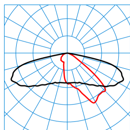
LIQ 50N-AB2L-LRA/22/26/32-722 4G1 ETDD (CLO initial value) TX778461
