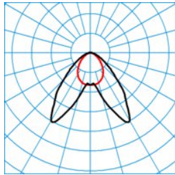
ELINE LDAW55-140 ML 840 L225 2 50
