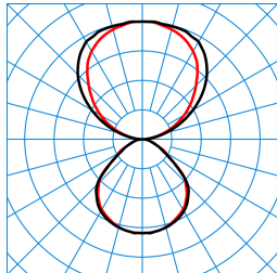
Luceos D/H1-L CDP 6700-840 ETDD 01 (Pendant ZS/ZST) TX547706
