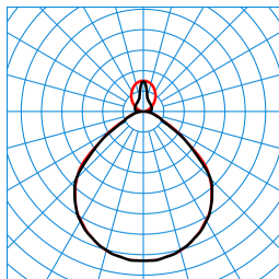
Luceos D/H1-L CDP 6700-840 ETDD 01 (Ceiling D1 ZD/01+EB3) TX547716
