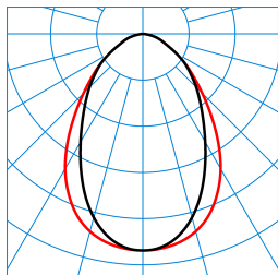
ArimoFit G2 Act M59 DW19 53-8 ETDD8 (ActDSU) TX376382
