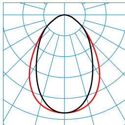
ArimoFit G2 Act M59 DW19 53-8 ETDD8 + ArimoFit G2 Sky M59-TS ZER (ActDSU) TX426800
