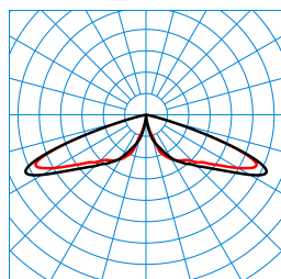
CS 19 100-RB6L/2200-730 2G1S ETDD (CLO initial value) TX299931
