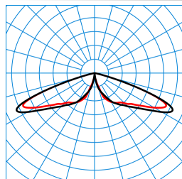
CS 19 100-RB6L/2200-730 2G1S ETDD (CLO end value) TX299930
