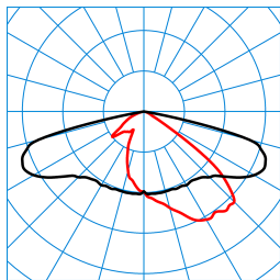
LIQ 70N-AB7L-LRA/10/12/135-730 12G1 ETDD (CLO end value) TX278275
