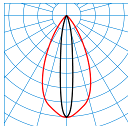
Altigo G2 C 60 SE6L/800-840 1G1P + VE IP66 24V DC 250W TX120435
