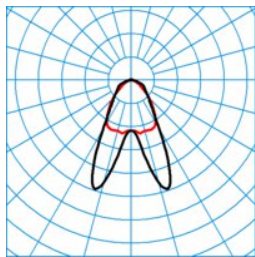
ELINE LDAN40-110 ML 865 L150 2 50 ■ C0 - C180
