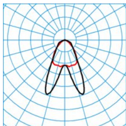
ELINE LDAN40-110 ML 865 L150 4 50 ■ C0 - C180
