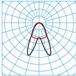
ELINE LDAN40-110 ML 865 L150 0 50 ■ C0 - C180
