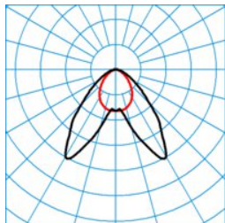
ELINE LDAW55-140 ML 865 L225 0 50
