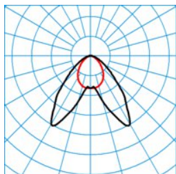
ELINE LDAW55-140 ML 865 L225 4 50
