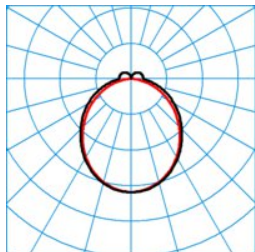
ELINE HE DSL35-110 ML 830 L150 0 50
