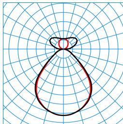
Opendo H2-L PW19 57-830 ETDD +LLWM 01 TX277388
