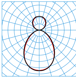
SFlow H3-L MRWD LED6400-840 ETDD LLWS 01 TX770547
