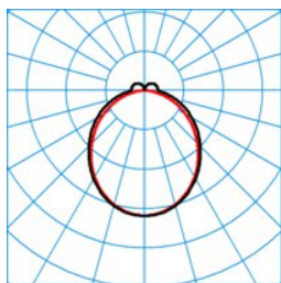
ELINE HE DSL55-140 ML 865 L225 2 50
