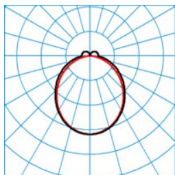
ELINE HE DSL55-140 ML 865 L225 4 50
