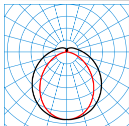
So-TubeAct G3 D/H4 DW 40 ETDD 05 (ACTDICW) TX773710
