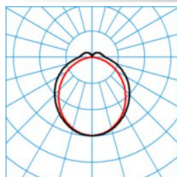
ELINE DL120 830 L150 1 50
