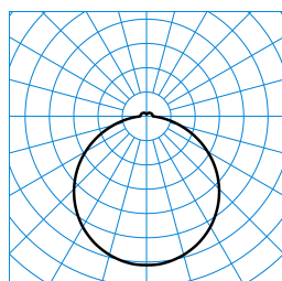
Olisq Act RWD4 DW 60 ETDD8 PC (ActDCW) TX375514 ■ C0 - C180 ■ C90 - C270
