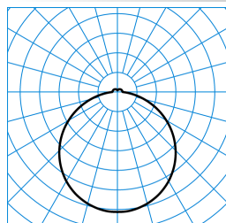
Olisq Act RWD4 DW 60 ETDD8 PC (ActDWW) TX376335 ■ C0 - C180 ■ C90 - C270
