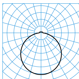
Olisq Act RWD4 DW 60 ETDD8 PC (ActDSU) TX375790 ■ C0 - C180 ■ C90 - C270
