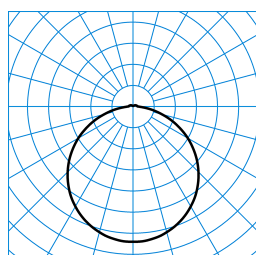
Olisq Act RWD4 DW 60 ETDD8 PC + Olisq RWD4 C 01 (ActDWW) TX427010 ■ C0 - C180 ■ C90 - C270
