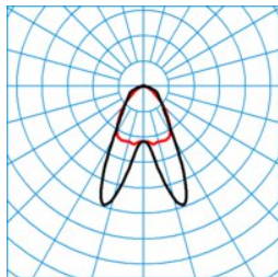
ELINE HE LDAN40-120 ML 840 L150 4 20 ■ C0 - C180
