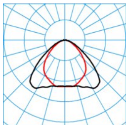
ELINE LVW40-110 ML 865 L150 4 50
