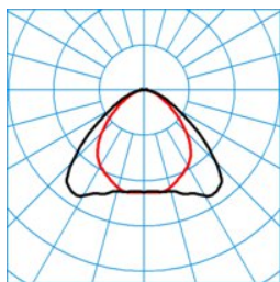
ELINE LVW40-110 ML 865 L150 2 50
