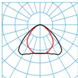
ELINE LVW40-110 ML 865 L150 0 50
