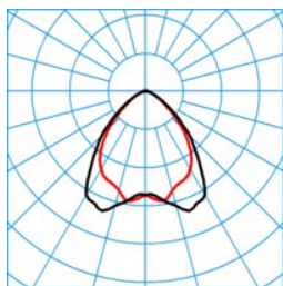
ELINE HE LW60-160 ML 830 L225 2 50 ■ C0 - C180
