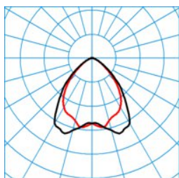
ELINE HE LW60-160 ML 830 L225 0 50 ■ C0 - C180
