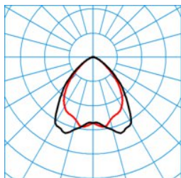
ELINE HE LW60-160 ML 830 L225 4 50 ■ C0 - C180
