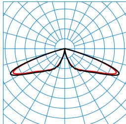
CS 19 100-RB6L/3800-730 4G1S ETDD (CLO end value) TX300111
