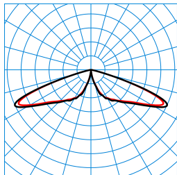
CS 19 100-RB6L/3800-730 4G1S ETDD (CLO initial value) TX300112
