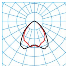
ELINE LW55-140 ML 830 L225 0 50
