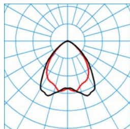
ELINE LW55-140 ML 830 L225 4 50
