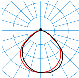
Luceos D/H2-L CDP-A 6500-830 01 (Pendant ZS/ZST) TX194610
