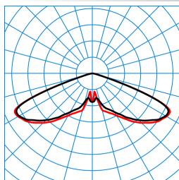
Publisca P2-RB6L/3200-730 4G1S TX047829
