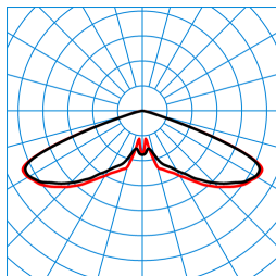
Publisca P2-RB6L/3200-730 4G1S ETDD (CLO initial value) TX300813
