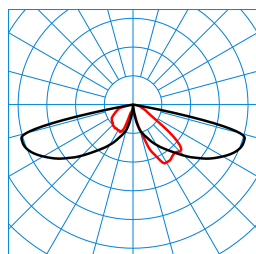
CS 19 100-AB2L/1650-740 2G1S ETDD (CLO initial value) TX299969
