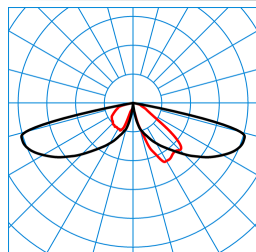
CS 19 100-AB2L/1650-740 2G1S ETDD (CLO end value) TX299968
